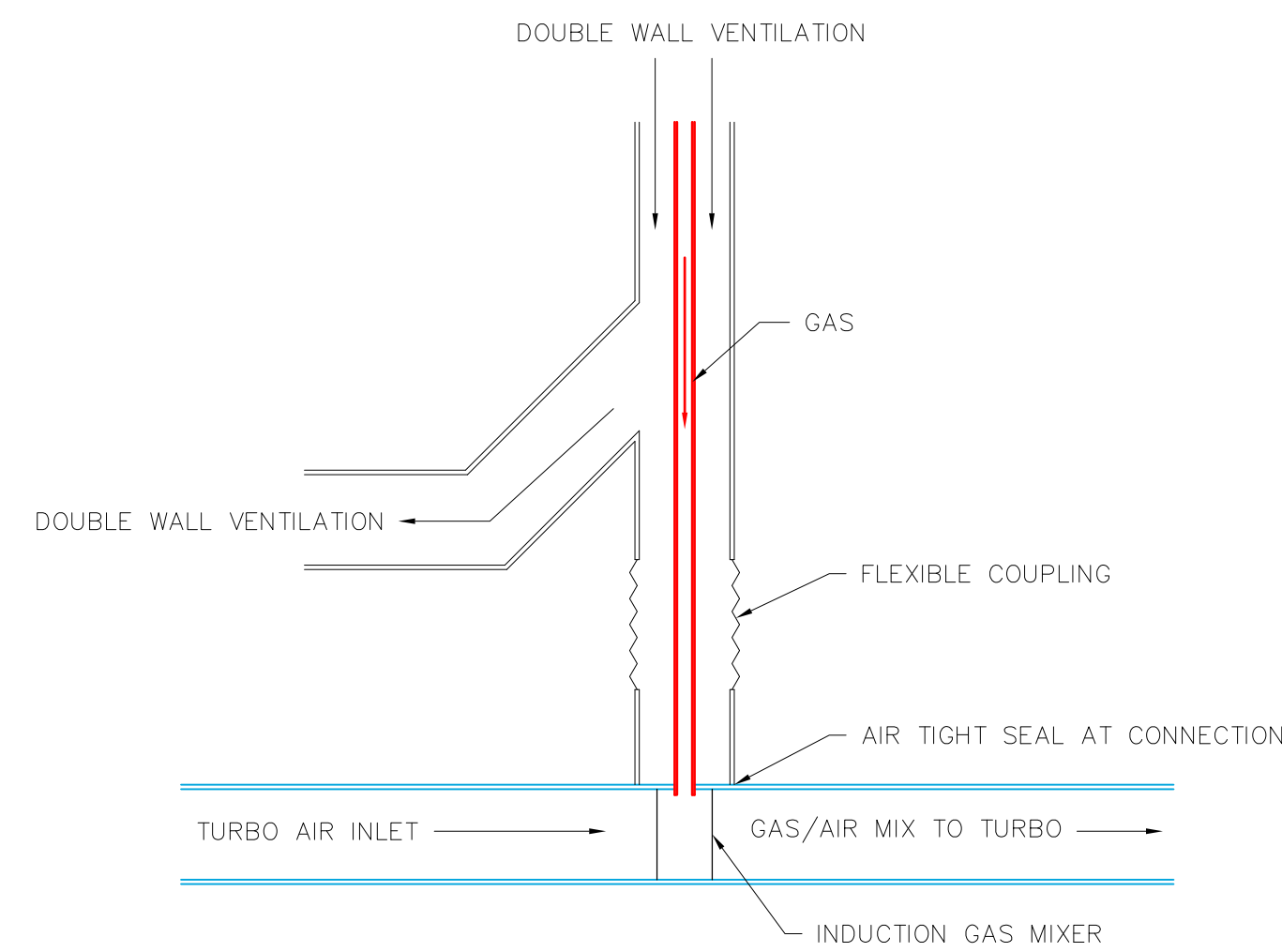
DETAIL 7-C PRELIMINARY INJECTION INLET SKETCH SCALE: 1"=1'-0"
